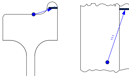
AP probe: Radial defect detection in wheel flange
