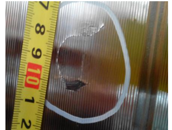
Crack with 25mm length and 30mm width, 5mm below the wheel rim tread
